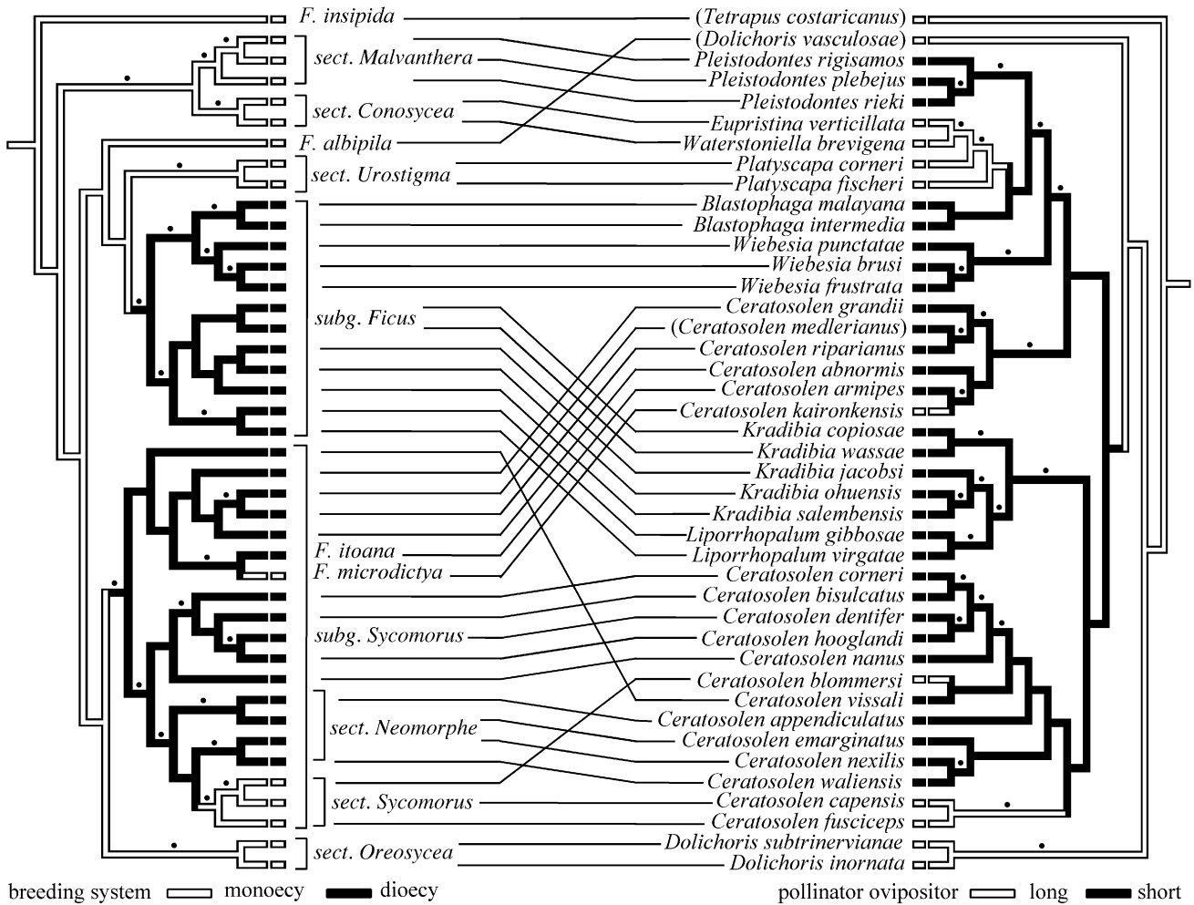
FIGURE 3. Fig and pollinator phylogenies indicating current associations and ancestral reconstructions of fig breeding systems and pollinator ovipositor lengths. Most-parsimonious trees for 42 fig species and their pollinators are based on separate analyses of nrDNA and mtDNA sequences, respectively (Weiblen, 2000, 2001). Bootstrap values >70\% are indicated by dots above the branches. Brackets mark some Ficus sections and subgenera, and three substituted pollinators are indicated in parentheses.
